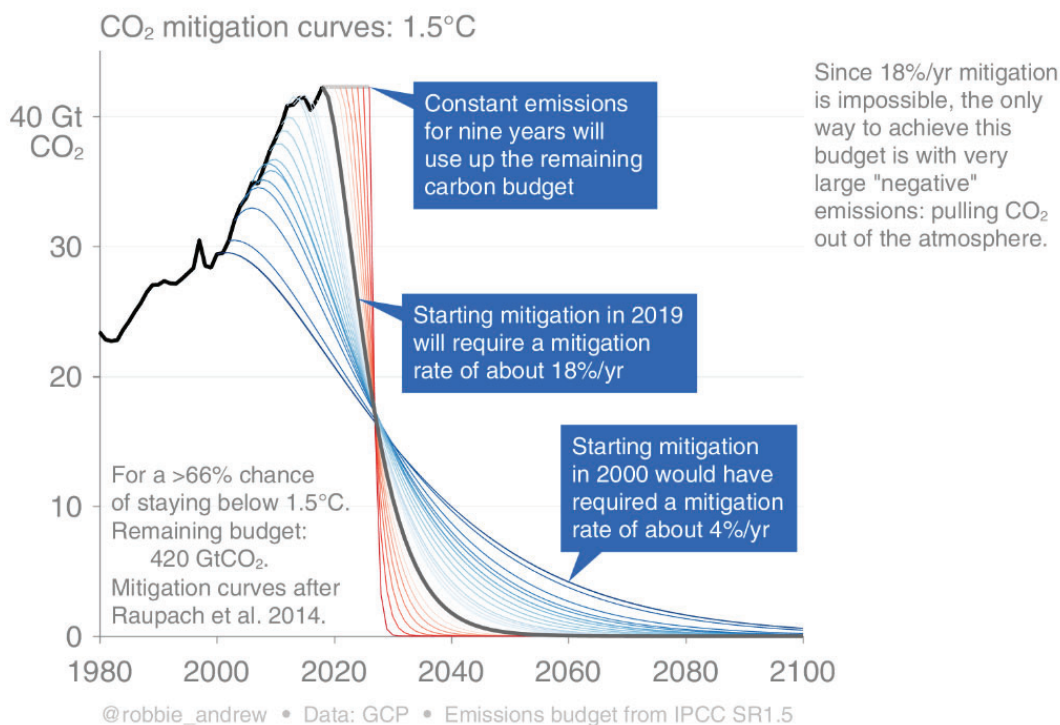
Figure 1 Emissions budget and pathways from IPCC SR1.5 2
