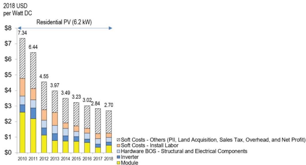
Figure 6 U.S. Solar Photovoltaic System Cost Benchmark 11
