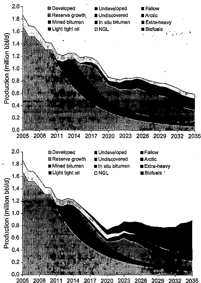
Fig. 4. Production in the United Kingdom in the LCS (top) and LCS-noCCS (bottom) scenarios split by category.
