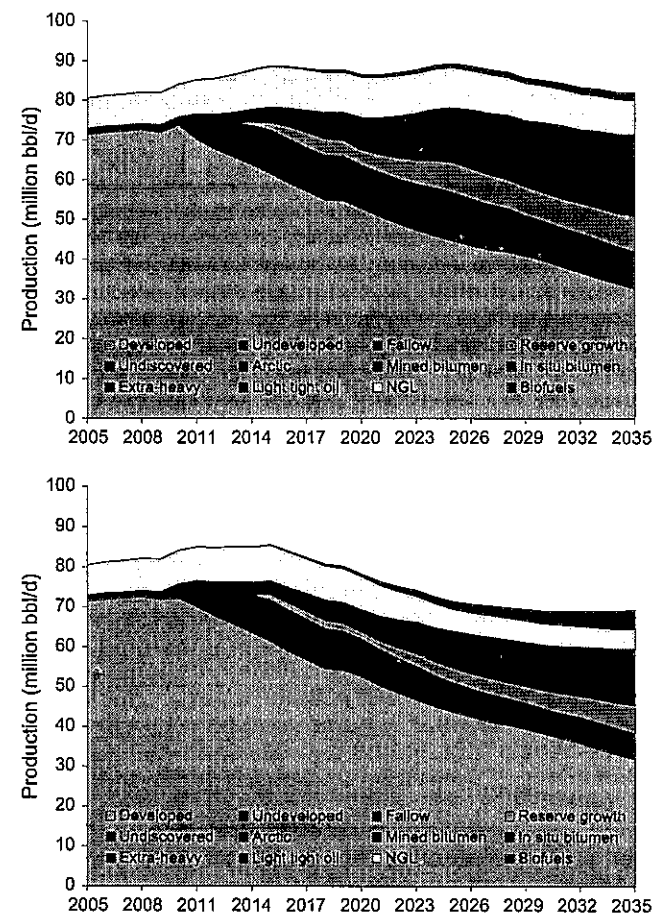
Fig. 2. Global production in LCS (top) and LCS-noCCS (bottom) split by resource category.
