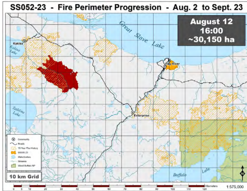
Figure 6: SS052-23 Wildfire Progress August 12-15, 2023. Produced by ECC.
