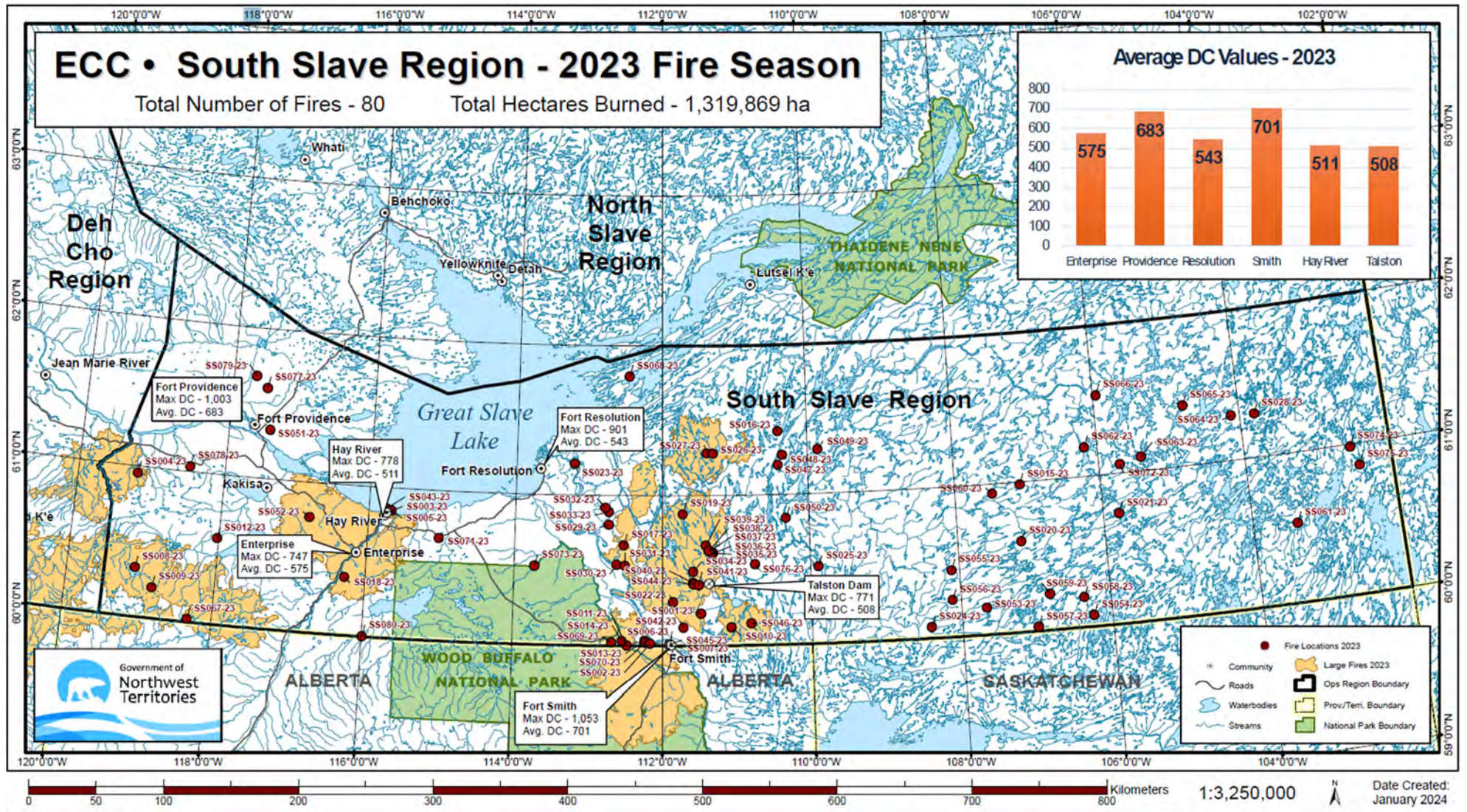
Figure 3: South Slave Region 2023 Fire Season. Includes noteworthy wildfires and drought codes (DC). Produced by ECC.
