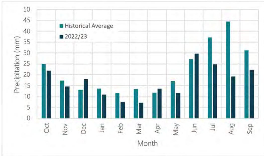
Figure 5: NWT 2022/2023 Monthly Precipitation Anomalies vs. Historical Average
