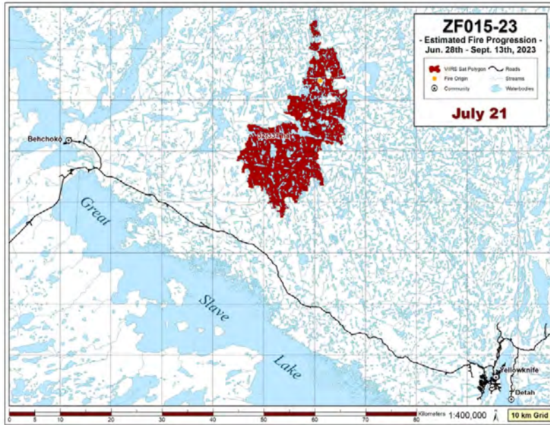
Figure 8: ZF015-23 Wildfire Progress July 21-28, 2023. Produced by ECC.
