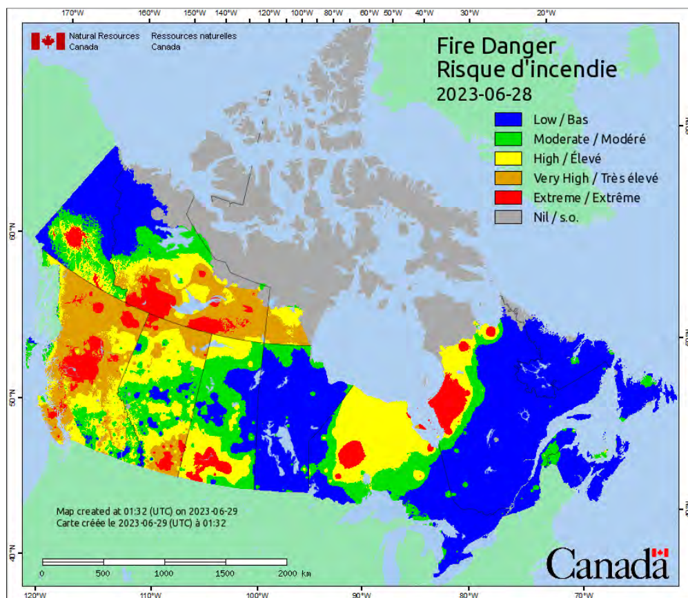
Figure 1: Wildfire Danger for June 28, 2023.
