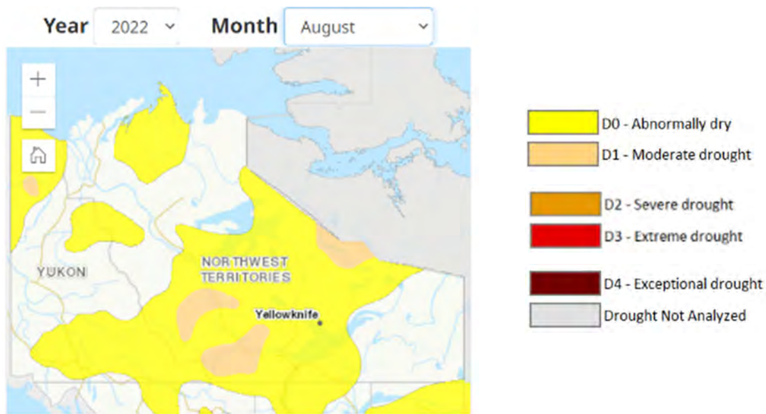
Figure 4: NWT Drought Conditions (August 2022) 7
