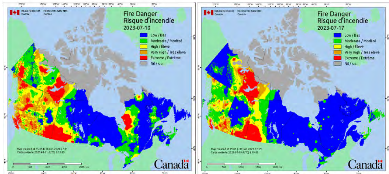
Figure 7: Wildfire Danger for July 17, 2023
