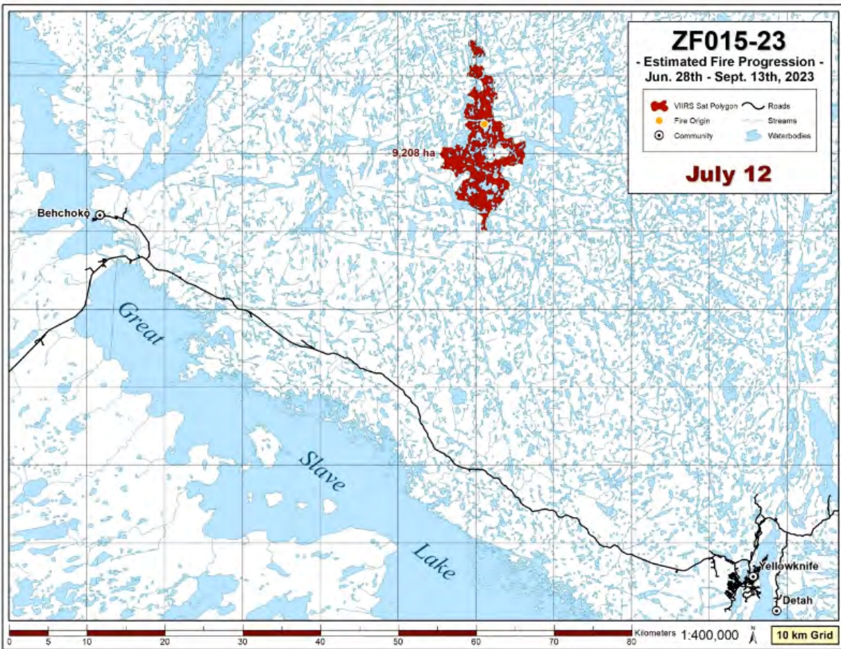
Figure 4: ZF015-23 Wildfire Progress. July 12, 2023. Produced by ECC.
